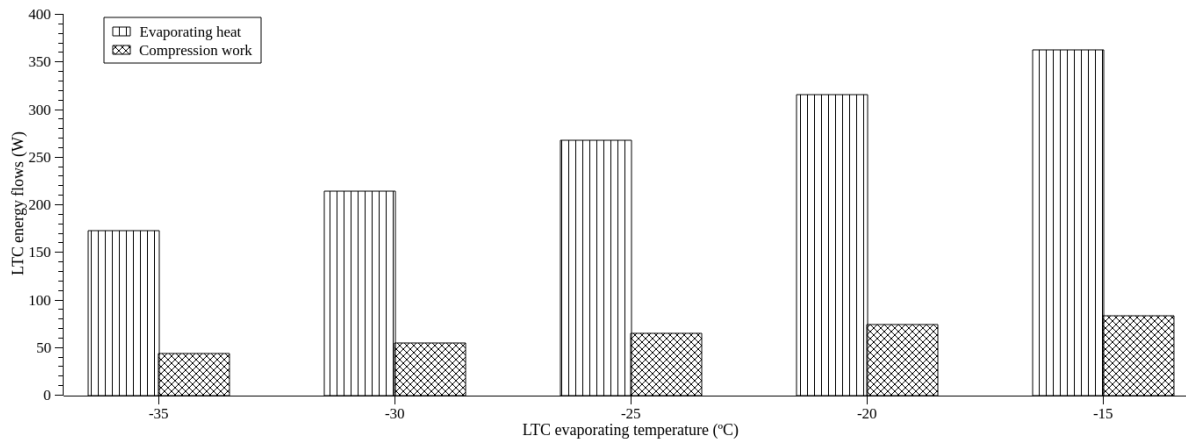
Figure 4. LTC input energy flows.
