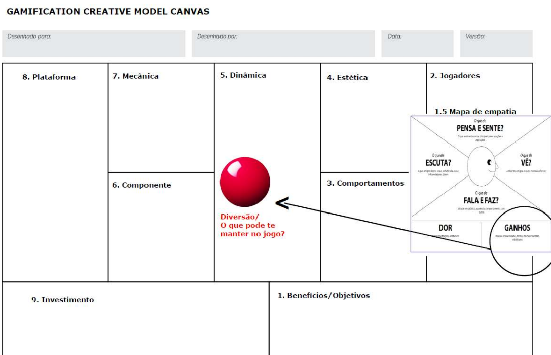
Figura 1 - Framework GCMC
